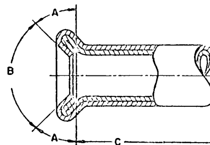
FIG. 2 Double-Flare Test
